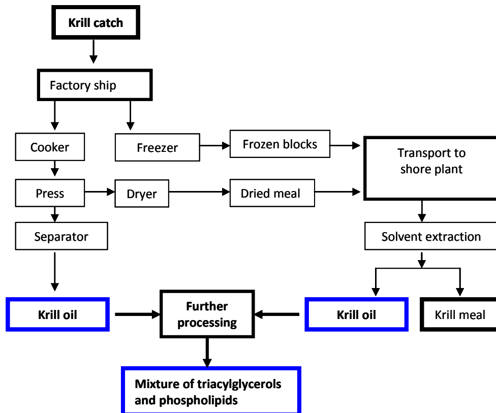
Figure 2.4.1: Overview of processing of krill to oil ( adopted from Bimbo, 2007 ). Krill is pumped alive onboard the factory trawler. The catch is either deep frozen onboard or directly produced to krill meal, resulting in dried meal with high fat content and an oil fraction rich in triacylglycerols. The krill meal can then be transported to a shore side facility where solvent extraction methods can be used to extract oil rich in phospholipids and produce a high-protein meal. The deep frozen krill is crushed and subjected to solvent extraction to obtain oil. The lipid extract is filtrated to remove proteins and krill material, and solvent and residual water are removed by evaporation.
